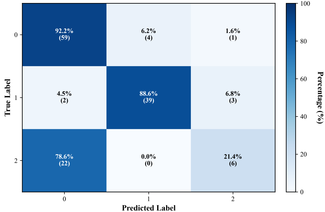
(a) 3-Expansion FLANN
